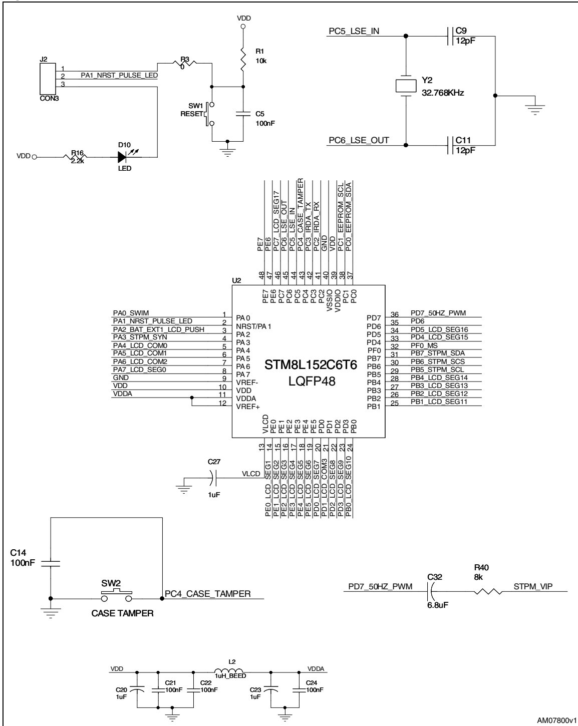
Figure 1. Microcontroller schematic
