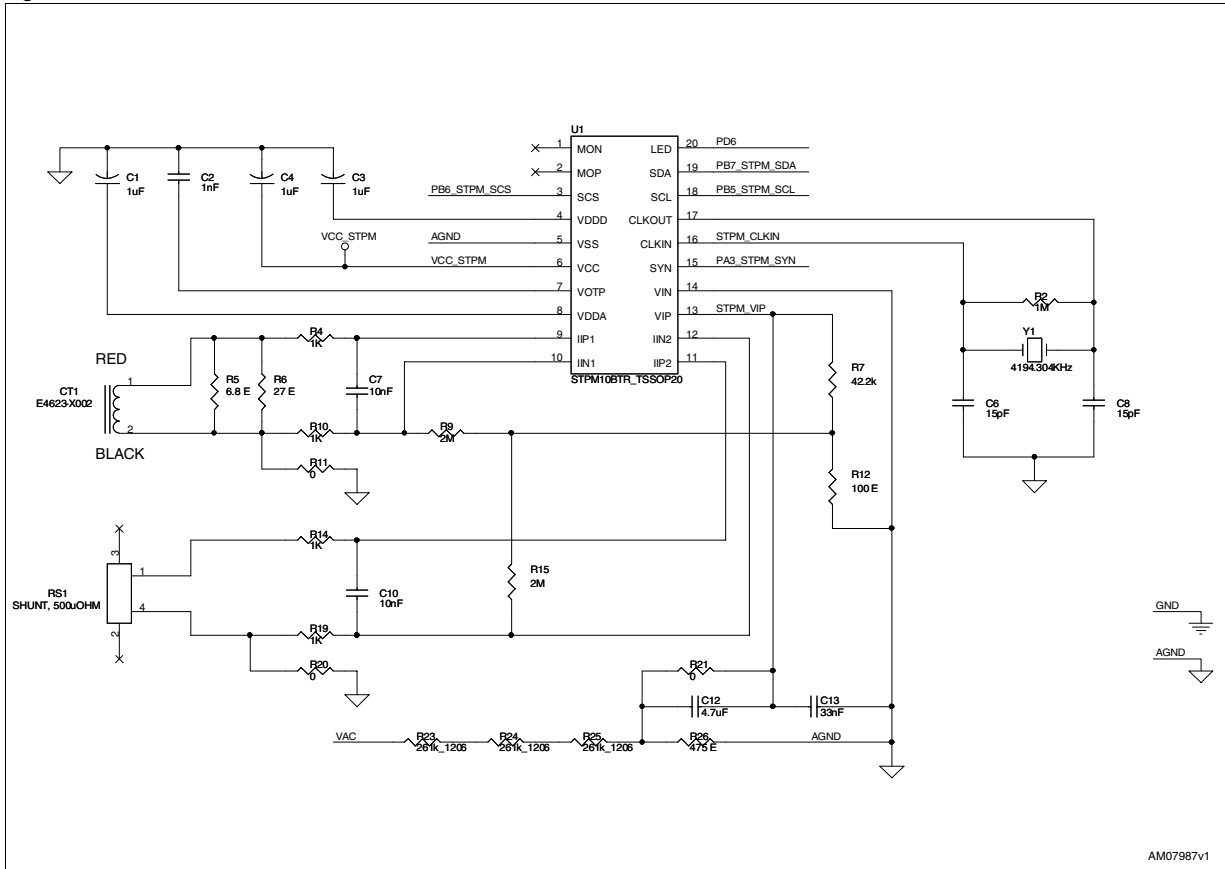
Figure 4. STPM schematic
