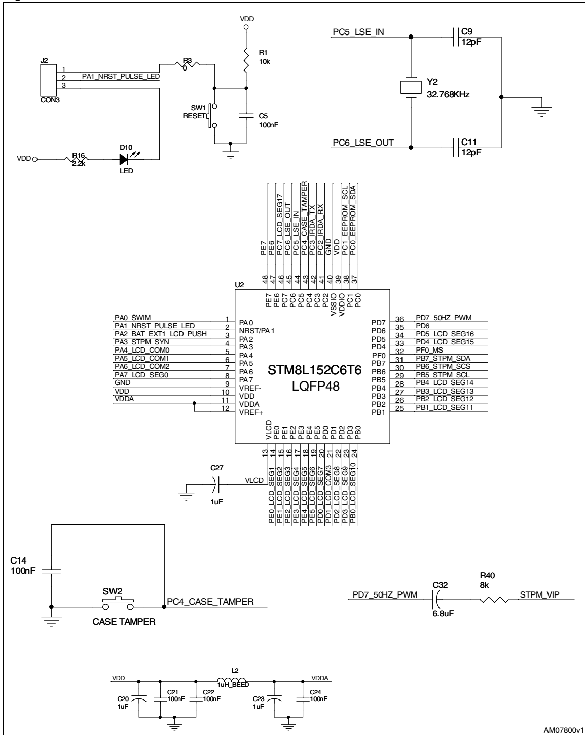
Figure 8. Microcontroller schematic
