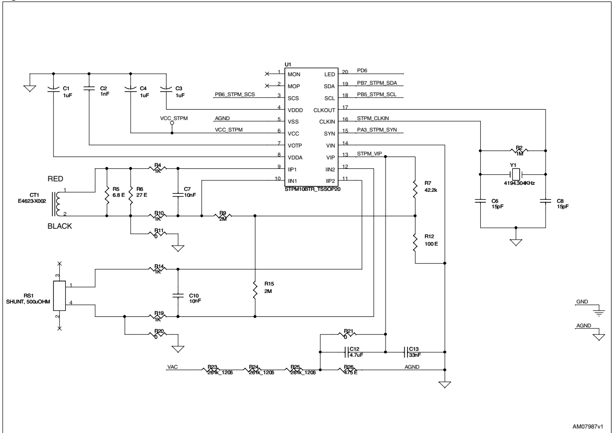
Figure 11. STPM schematic
