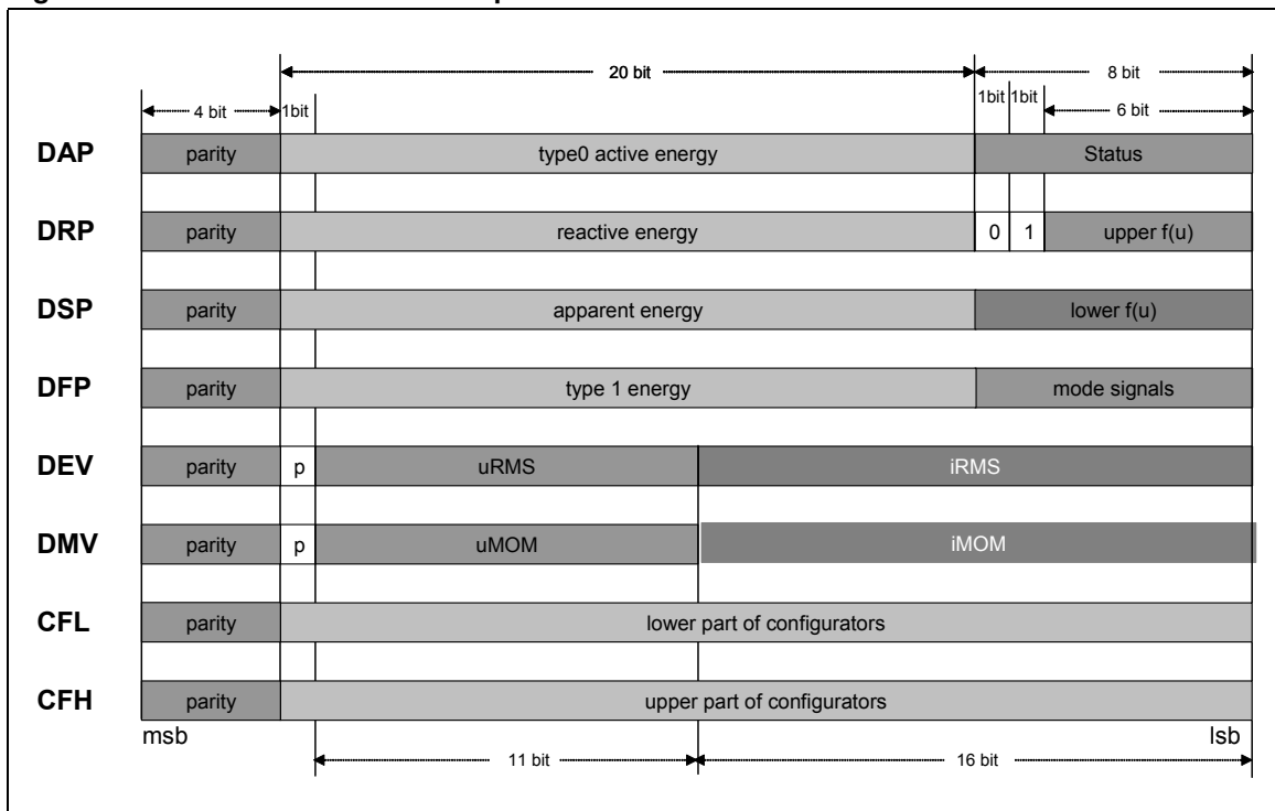
Figure 21. STPM10 data records map
