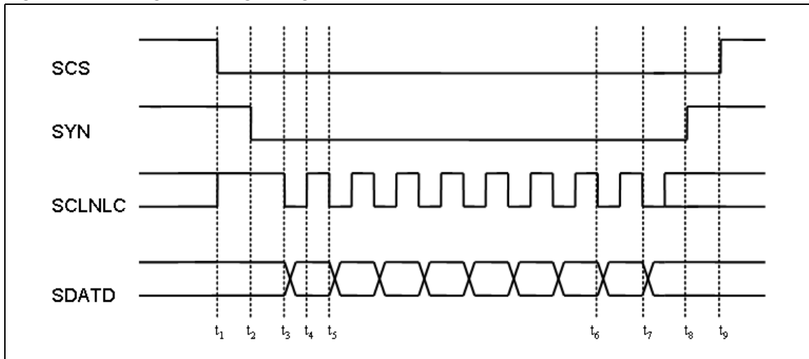
Figure 25. Timing for writing configuration and mode bits
