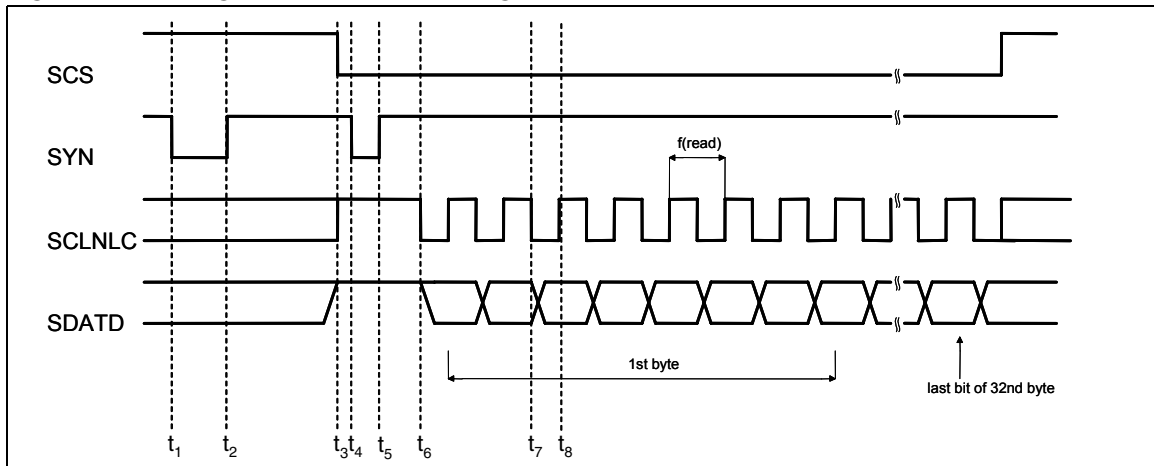
Figure 24. Timing for data record reading
