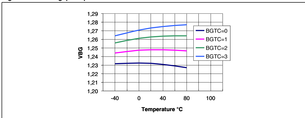
Figure 17. Band-gap temperature variation
