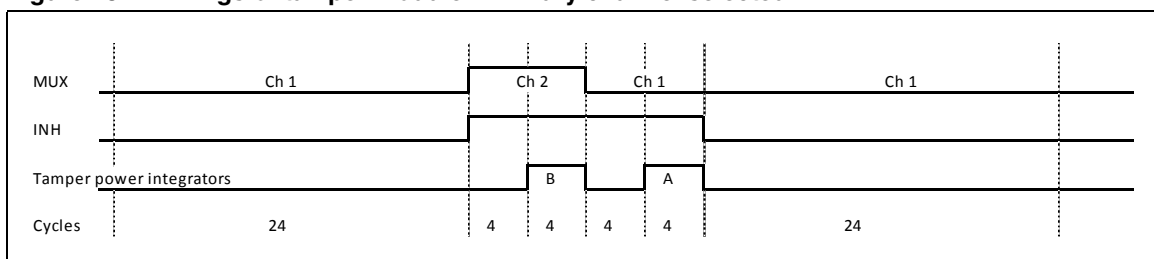
Figure 18. Timings of tamper module - Primary channel selected
