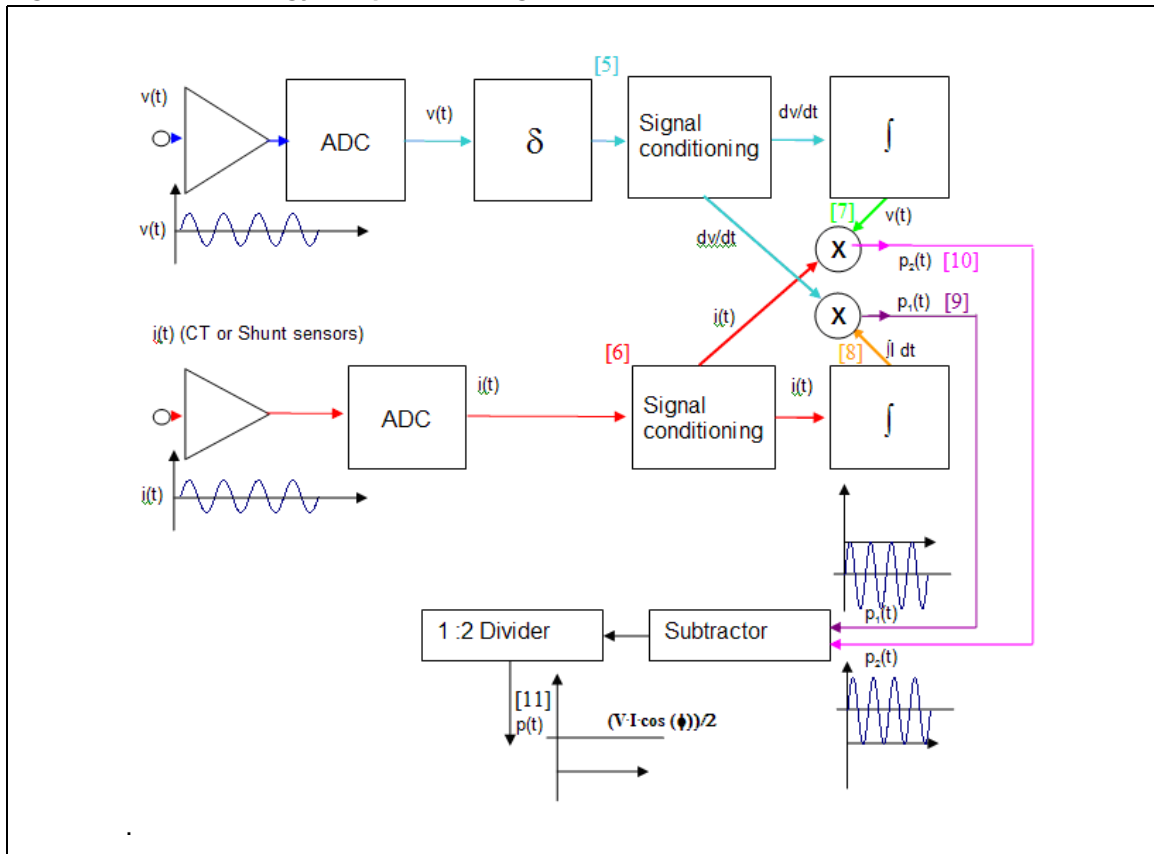
Figure 26. Active energy computation diagram
