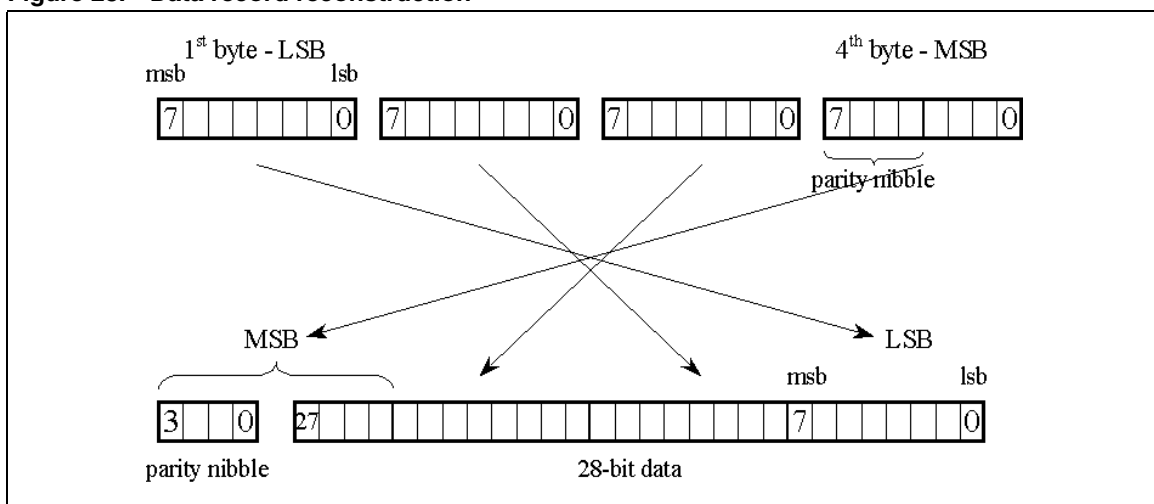
Figure 23. Data record reconstruction
