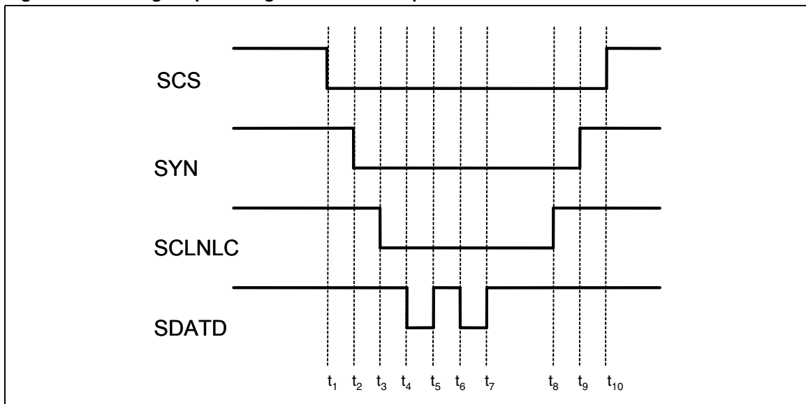
Figure 22. Timing for providing remote reset request (1)
