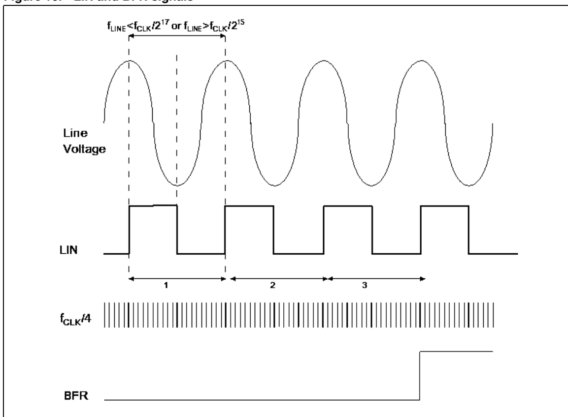
Figure 16. LIN and BFR signals
