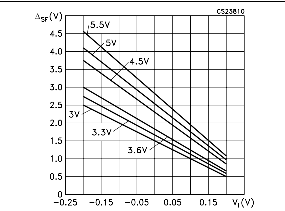
Figure 8. Voltage channel linearity at different V_{CC} voltages
