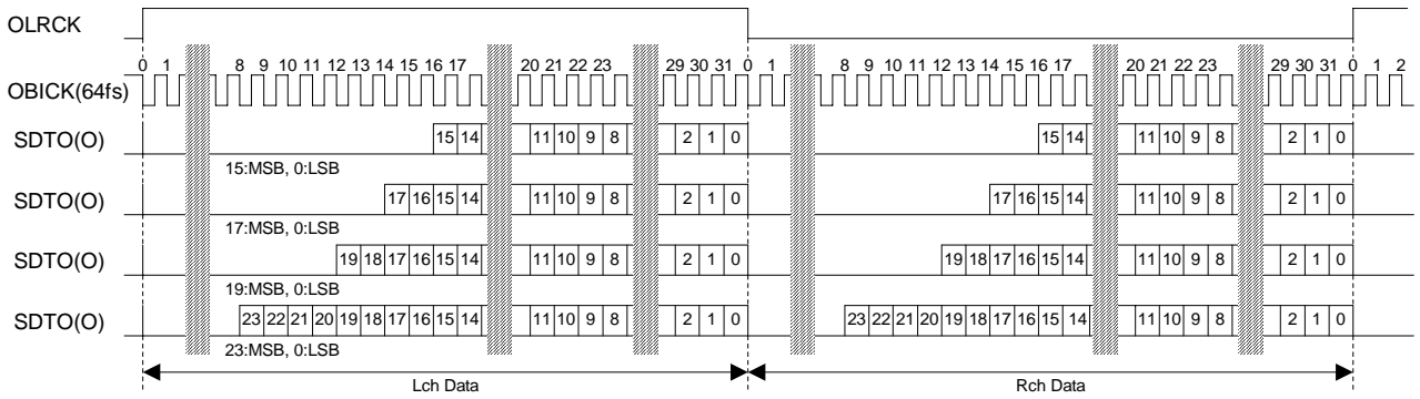
Figure 6. LSB Timing
