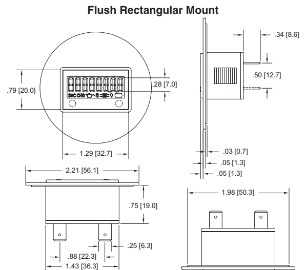
Panel Cutout: 1.45" [36.8mm] x 0.95" [24.1mm] Maximum Panel Thickness: 0.375" [9.5mm]
