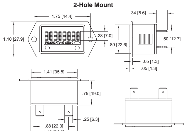
Panel Cutout: 1.45" [36.8mm] x 0.95" [24.1mm]
