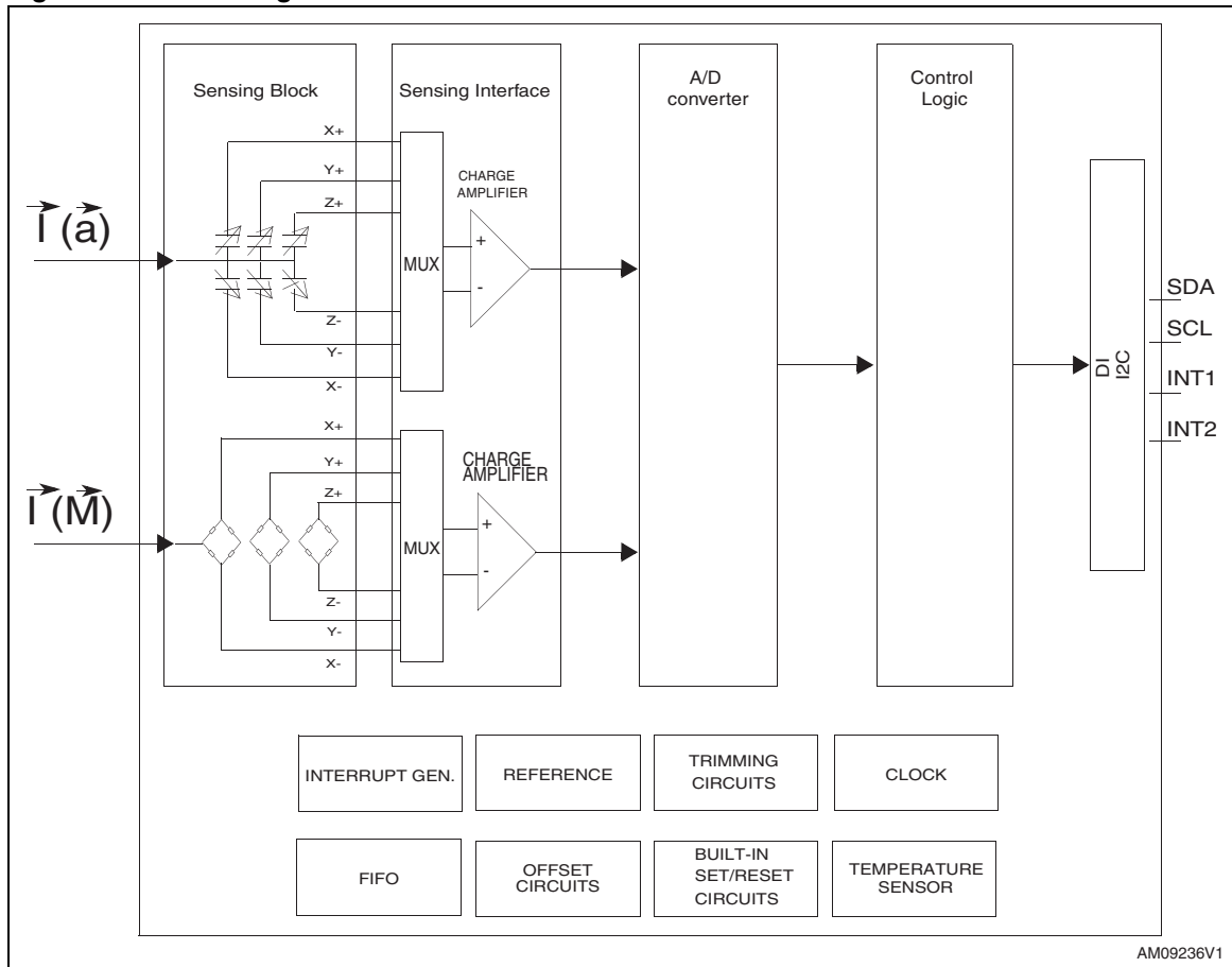
Figure 1. Block diagram
