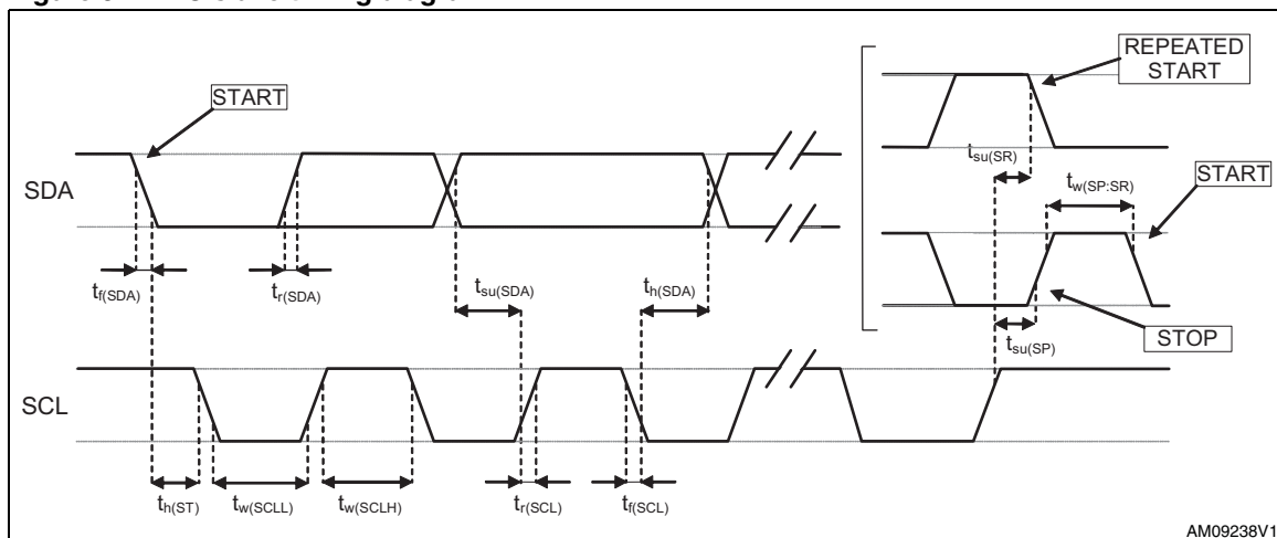
Figure 3. I 2 C slave timing diagram (c)
