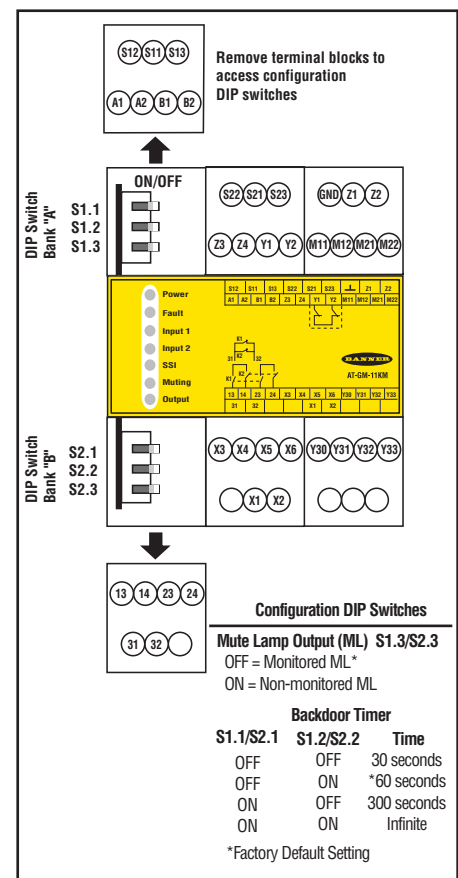
Figure 5. Backdoor Timer setup
