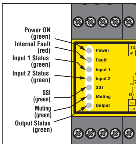
Figure 1. AT-..M-11KM status indicators
