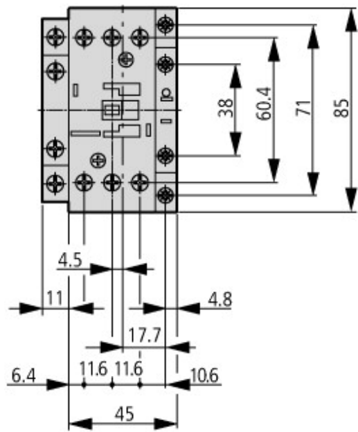
Contactor with auxiliary contact module
