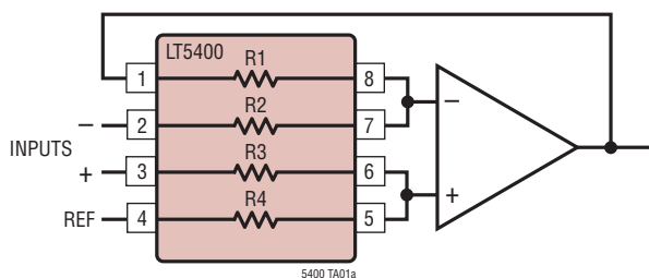
Difference Amplifier
