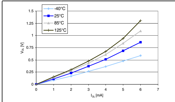
Figure 25. Typ. V_{OL} @ V_{DD} = 3.3\text{ V} (true open drain ports)
