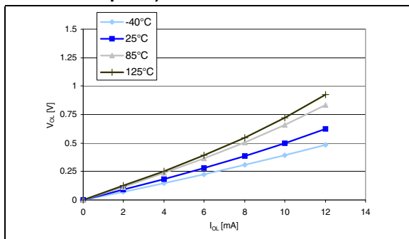
Figure 27. Typ. V_{OL} @ V_{DD} = 3.3\text{ V} (high sink ports)
