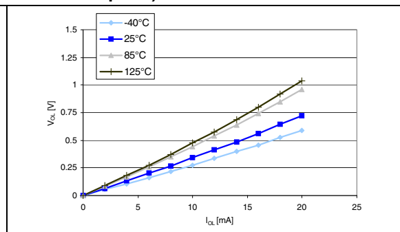
Figure 28. Typ. V_{OL} @ V_{DD} = 5.0\text{ V} (high sink ports)
