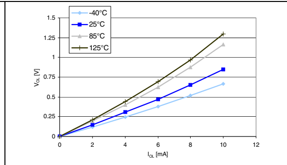
Figure 26. Typ. V_{OL} @ V_{DD} = 5.0\text{ V} (true open drain ports)
