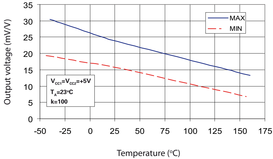
Output voltage versus temperature
