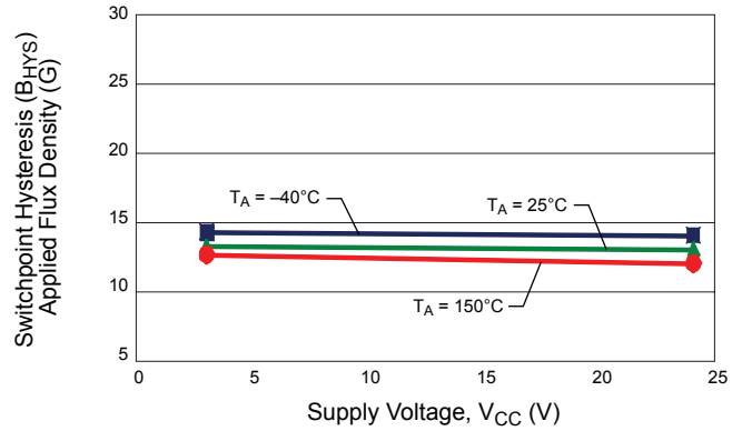
Average Hysteresis (North) versus Supply Voltage
