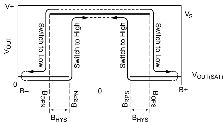
Figure 1. Switching behavior of omnipolar switches. On the horizontal axis, the B^+ direction indicates increasing south polarity magnetic field strength, and the B^- direction indicates increasing north polarity. This behavior can be exhibited when using a circuit such as that shown in figure 2.
