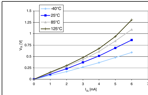
Figure 25. Typ. V_{OL} @ V_{DD} = 3.3 V (standard ports)
