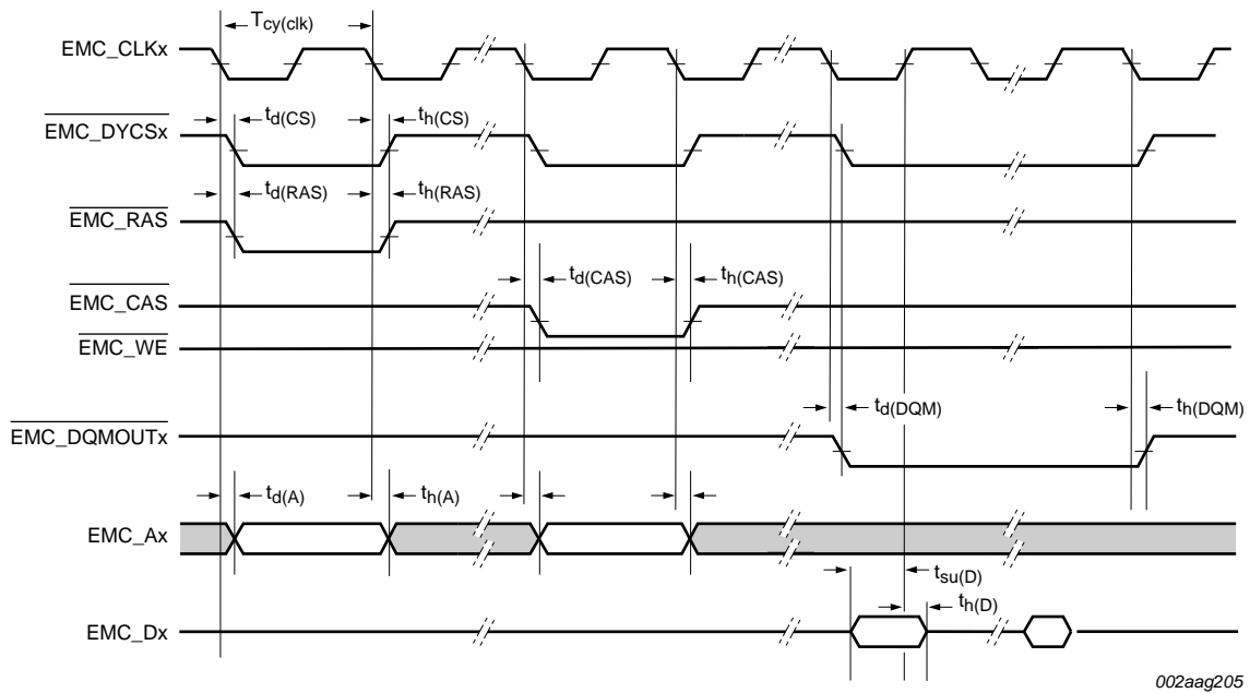
Fig 36. Dynamic external memory interface signal timing (read access)
