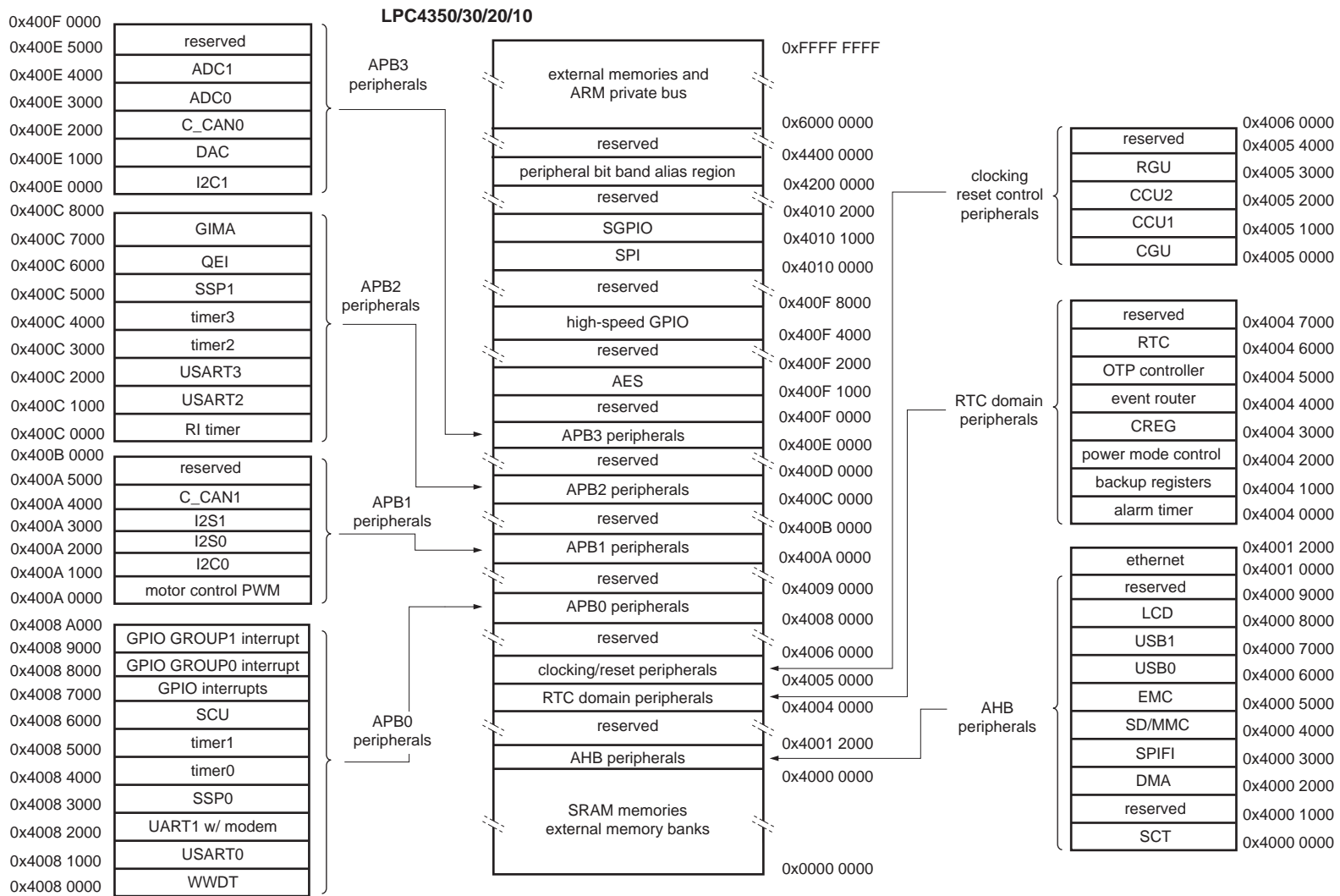
Fig 10. LPC4350/30/20/10 Memory mapping (peripherals)
