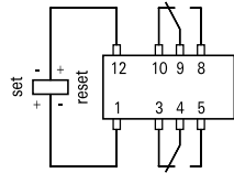
Bistable version, 1-coil
