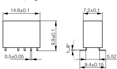
SMT, long terminals
