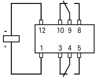
Monostable version
