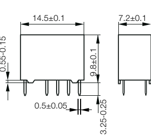
THT version
