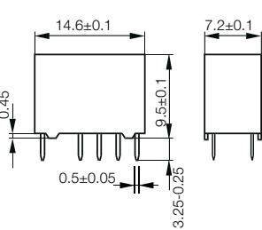
THT version
