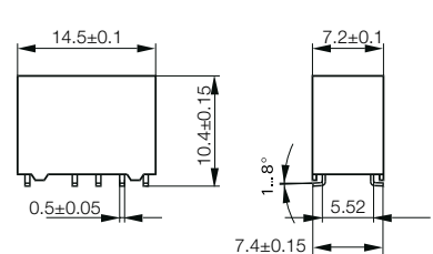
SMT, short terminals
