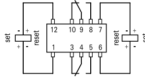
Bistable version, 2-coils
