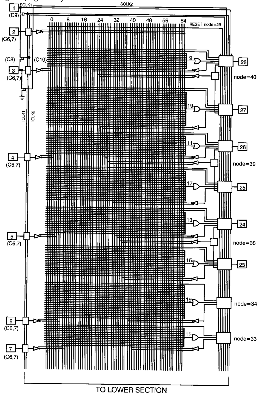
Block Diagram (Page 1 of 2)
