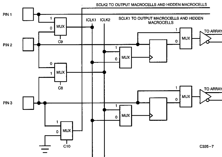
Figure 4. CY7C335 Input Cloning Scheme
