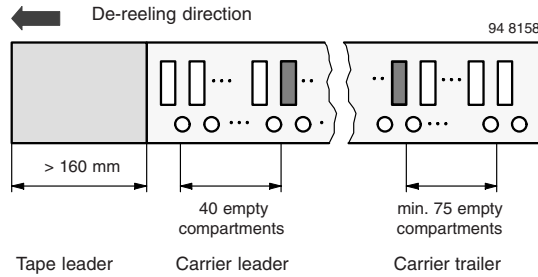
Figure 13. Beginning and End of Reel
