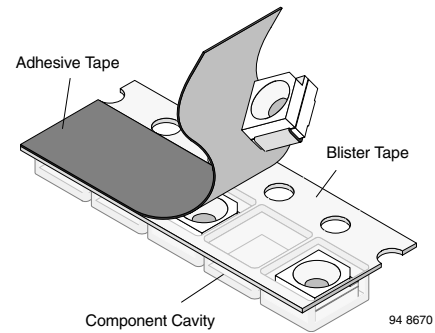
Figure 11. Blister Tape
