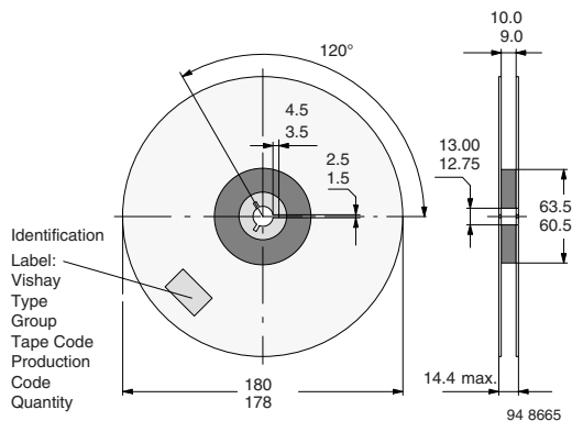
Figure 14. Dimensions of Reel
