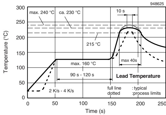
Figure 10. Lead Tin (SnPb) Reflow Solder Profile
