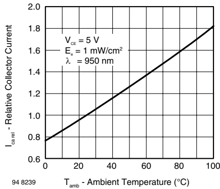
Figure 3. Relative Collector Current vs. Ambient Temperature
