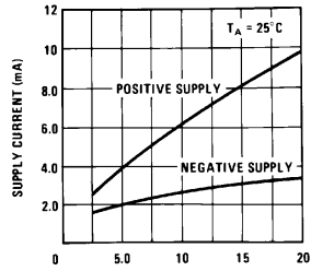
Supply Current
