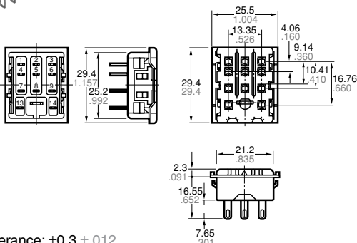
External dimensions
