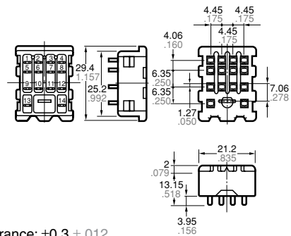
External dimensions
