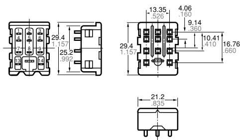
External dimensions
