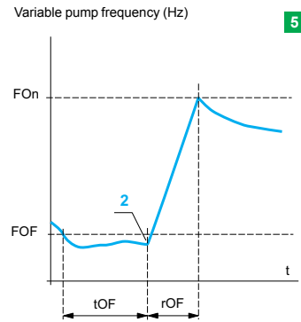
Auxiliary pump stop
