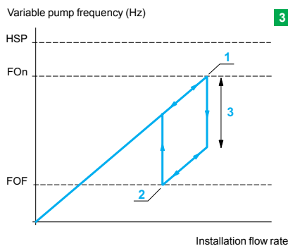
Single variable mode with auxiliary pump: hysteresis
