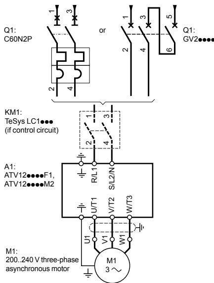
Motor starter with single-phase power supply
