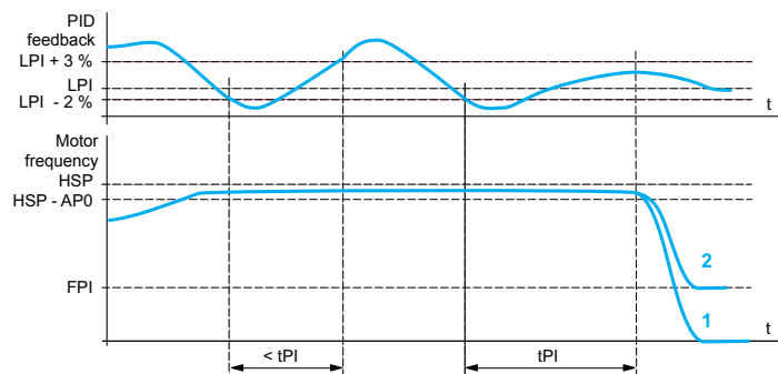
PID feedback supervision
