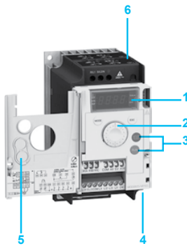
ATV12H075M2 with door on front panel open
