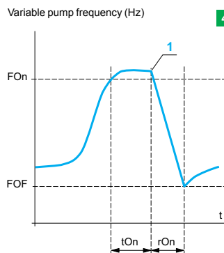
Auxiliary pump start
