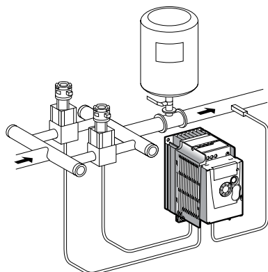
Single variable mode with auxiliary pump
