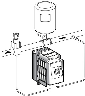
Single variable mode
