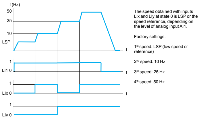
Example of operation with 4 preset speeds
