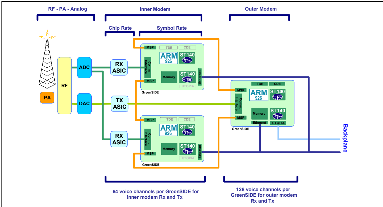
Figure 4. W-CDMA Node-B (1-Carrier, 128 voice users) - 3 chip-based
