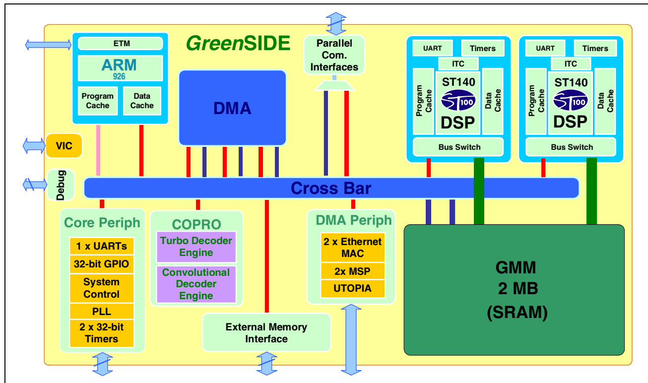
Figure 2. GreenSIDE ASSP Block Diagram
