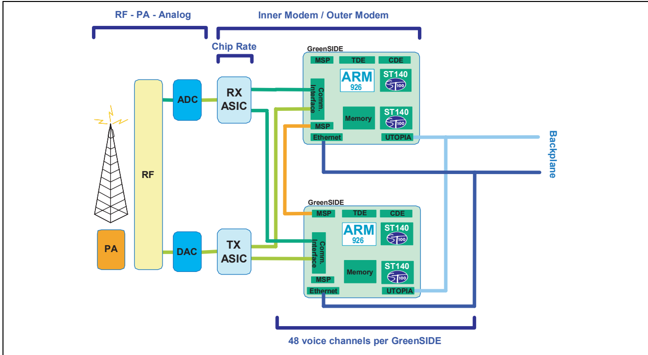
Figure 3. W-CDMA Node-B (1-Carrier, 96 voice users) - 2 chip-based
