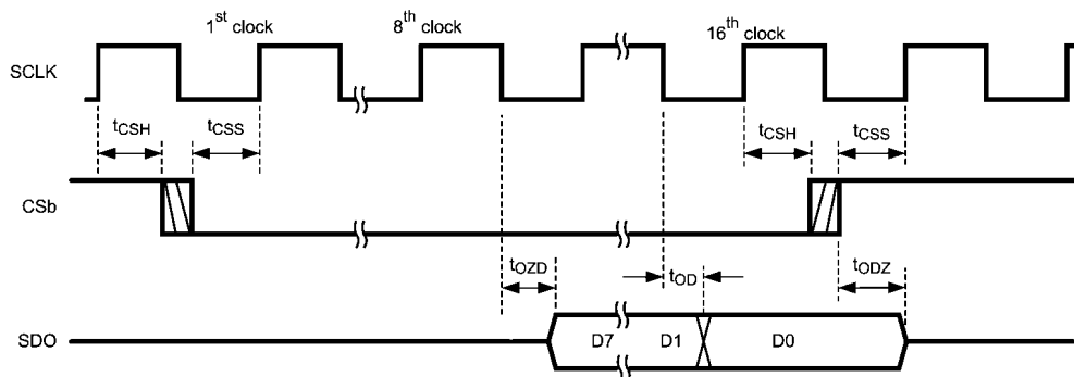
FIGURE 12. Read Timing
