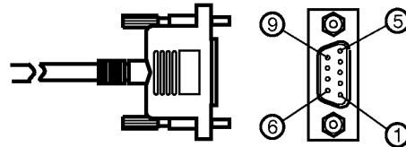
F10-VR4 RS-422 Cable: D-sub 9-pin connector (2 m)
