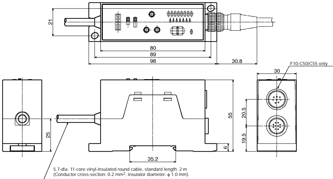
Mounting Dimensions
