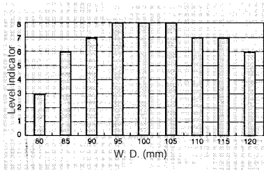
Distance Characteristics
