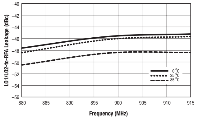
Figure 40. Channel A LO1-to-RF Leakage vs Frequency and Temperature
