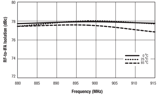
Figure 38. Channel A RF-to-IFA Isolation vs Frequency and Temperature
