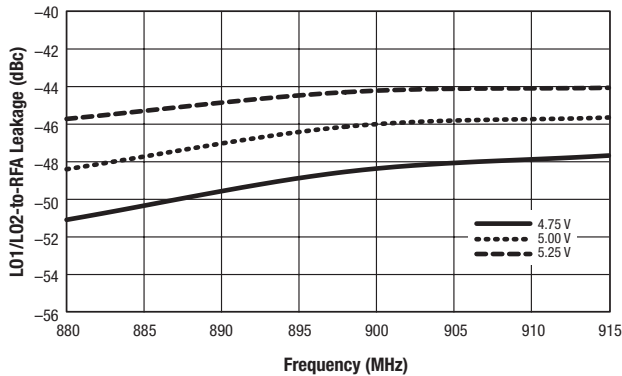
Figure 39. Channel A LO1-to-RF Leakage vs Frequency and Supply Voltage
