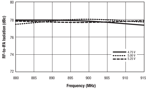
Figure 37. Channel A RF-to-IFA Isolation vs Frequency and Supply Voltage
