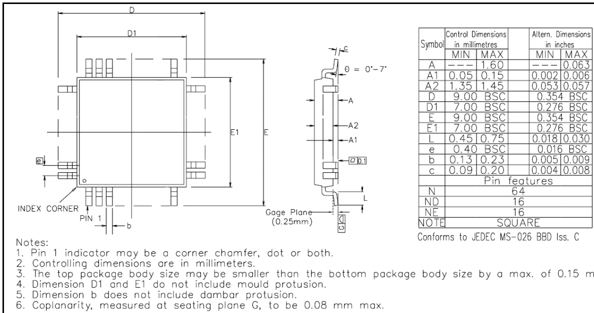
Figure 2 - Package dimensions
