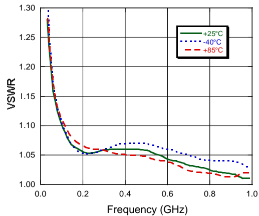
VSWR, 1000 pF
