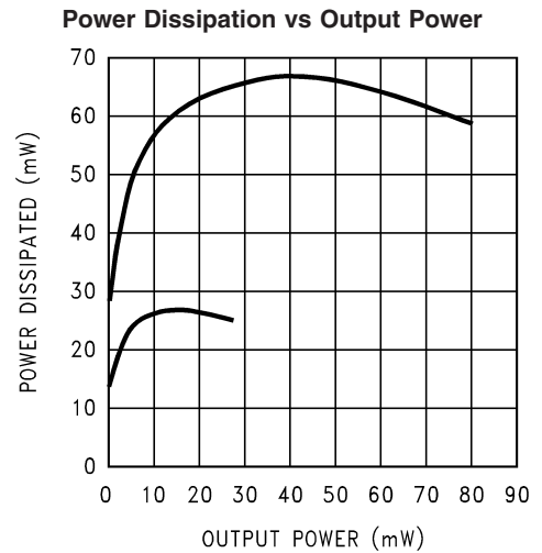
LHP, RHP; R_L = 32\Omega ; THD+N \leq 1\% Top- V_{DD} = 5V ; Bot- V_{DD} = 3V per channel
