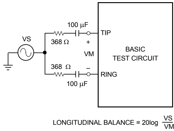
Figure 5. Longitudinal Balance
