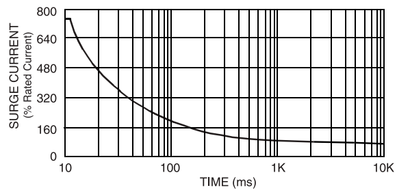
PEAK SURGE CURRENT VS DURATION FIGURE 3
