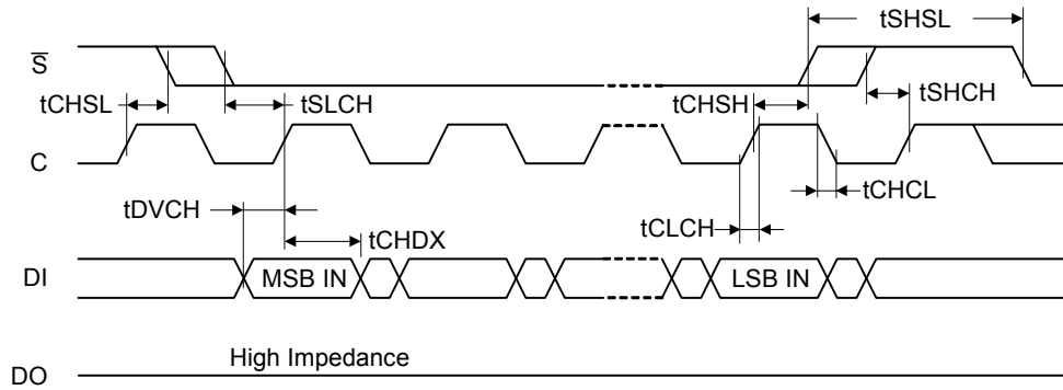
Figure 32. Serial Input Timing
