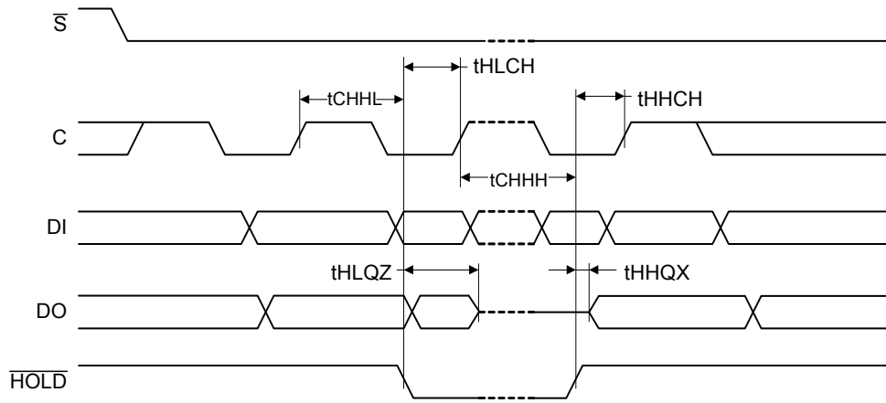
Figure 34. Hold Timing
