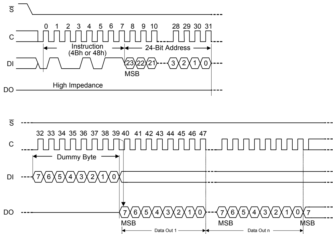
Figure 14. Read OTP (ROTP) instruction and data-out sequence
