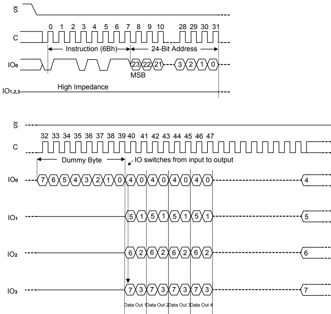
Figure 12. FAST_READ_QUAD_OUTPUT Instruction Sequence and Data-Out Sequence
