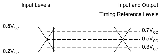
Figure 31. AC Measurement I/O Waveform
