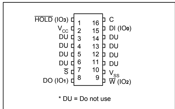
■ Figure 1b. SOP16 Connections
