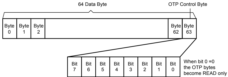
Figure 16. How to permanently lock the 64 OTP bytes
