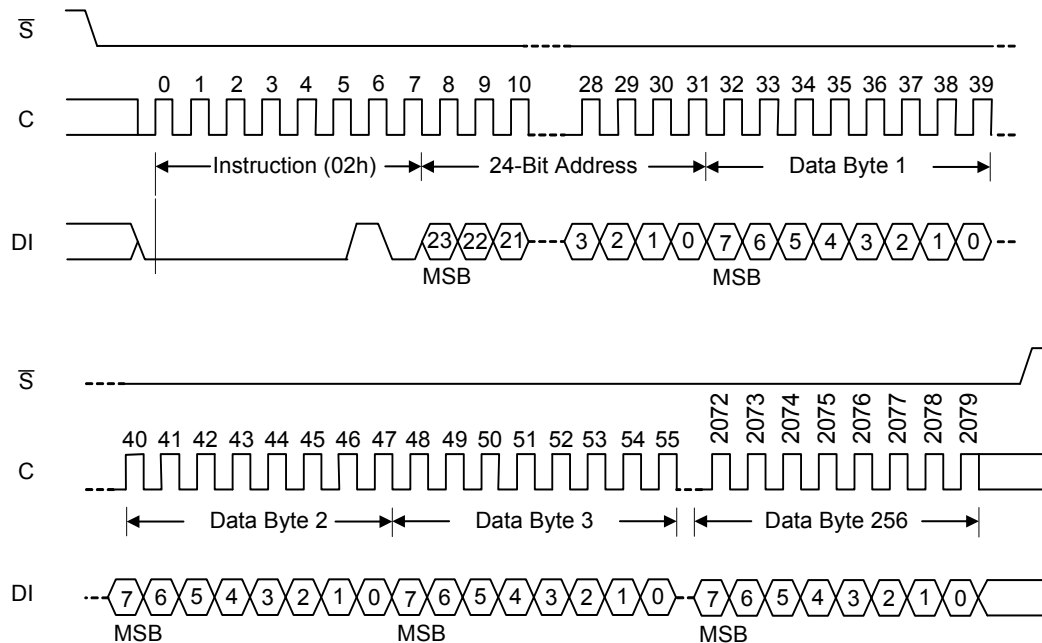
Figure 17. Page Program (PP) Instruction Sequence
