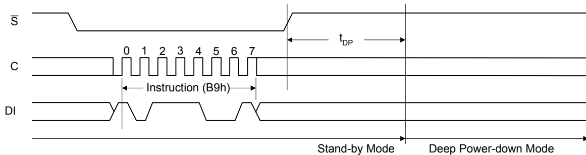
Figure 23. Deep Power-down (DP) Instruction Sequence
