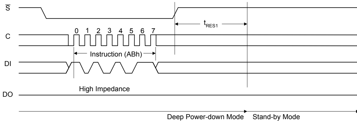
Figure 27. Release from Deep Power-down (RES) Instruction Sequence
