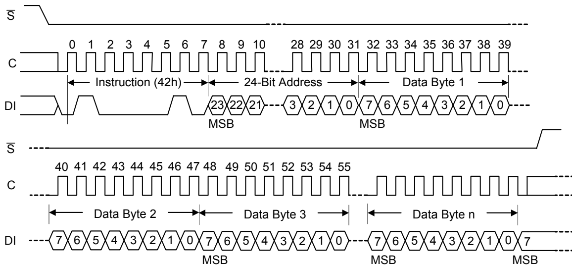
Figure 15. Program OTP (POTP) instruction sequence
