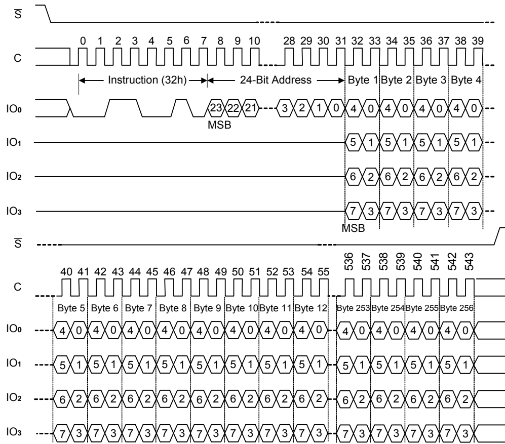
Figure 19. Quad Input Fast Program (QIFP) instruction sequence
