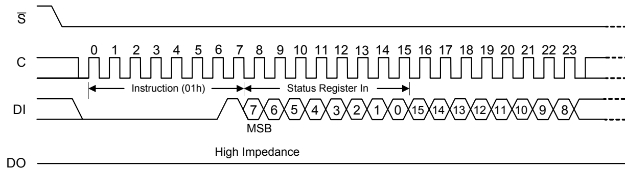
Figure 7. Write Status Register (WRSR) Instruction Sequence
