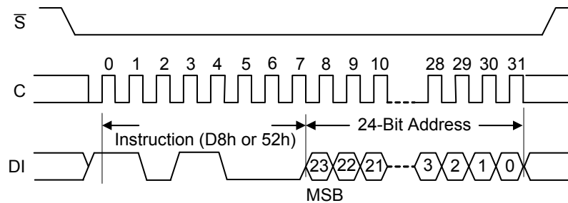
Figure 21. Block Erase (BE) Instruction Sequence
