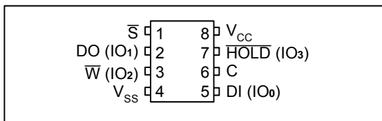
■ Figure 1a. SOP8, DIP8 Connections
