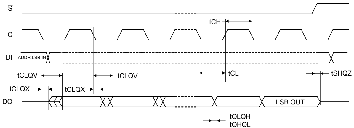
Figure 35. Output Timing
