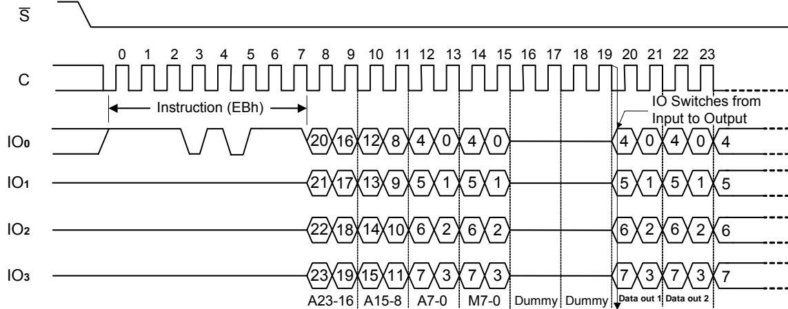
Figure 13-a. FAST_READ_QUAD_INPUT_OUTPUT Instruction and Data-Out Sequence (M5-4 ≠ 10h)
