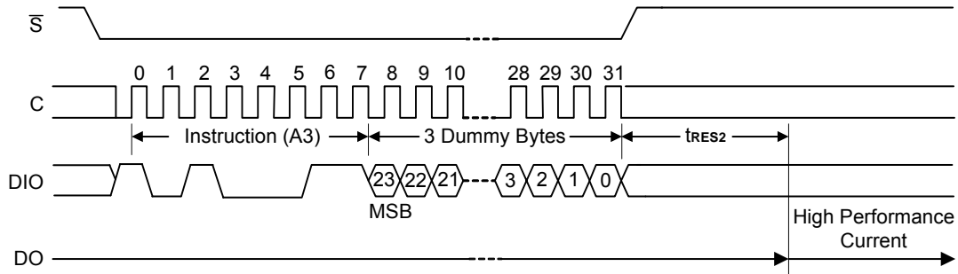
Figure 28. High Performance Mode Instruction Sequence
