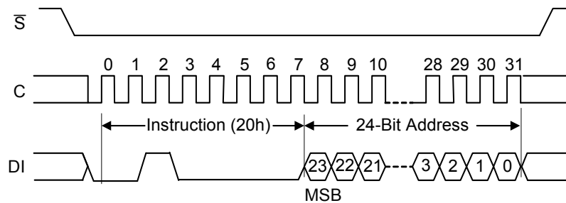
Figure 20. Sector Erase (SE) Instruction Sequence
