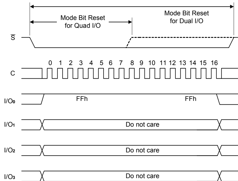
Figure 29. Continuous Read Mode Reset for Fast Read Dual/Quad I/O
