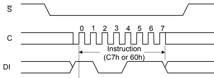
Figure 22. Chip Erase (CE) Instruction Sequence
