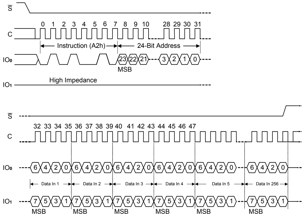
Figure 18. Dual Input Fast Program (DIFP) instruction sequence
