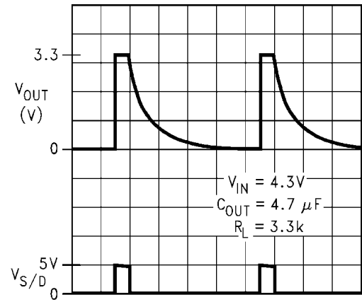
Turn-Off Waveform
