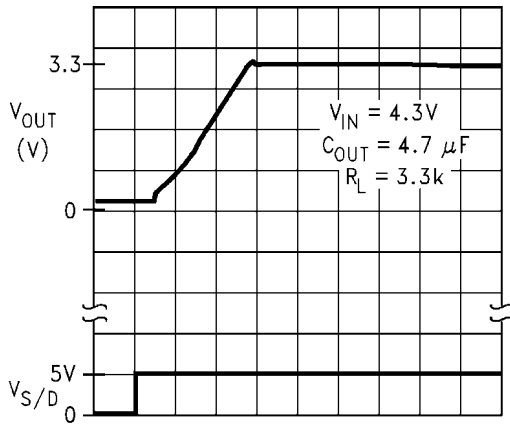
Turn-On Waveform
