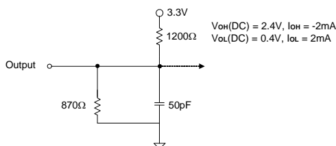
(Fig. 1) DC Output Load Circuit
