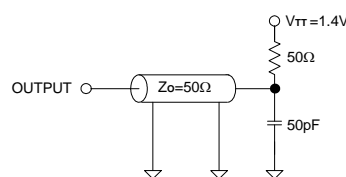
(Fig. 2) AC Output Load Circuit
