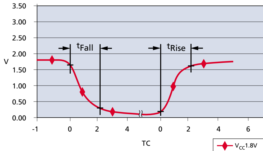
Figure 20: t_{\text{Fall}} and t_{\text{Rise}} (1.8V V_{\text{CC}} )
