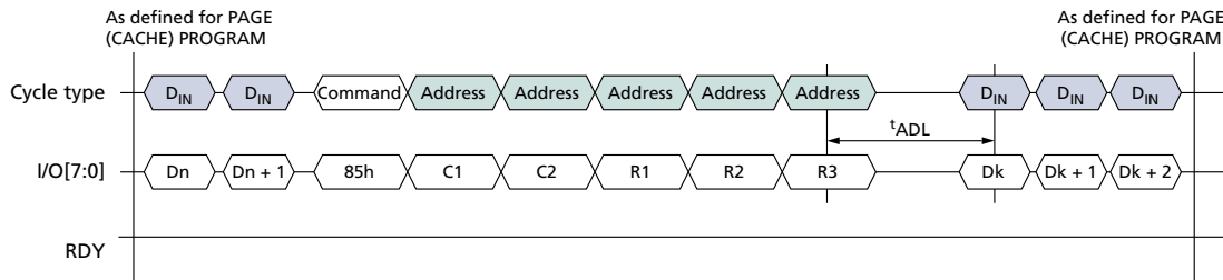
Figure 37: PROGRAM FOR INTERNAL DATA INPUT (85h) Operation
