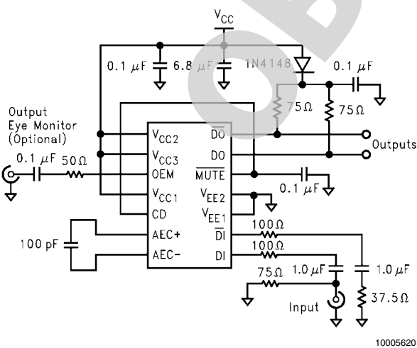
FIGURE 1. CLC014 Equalizer Application Circuit
