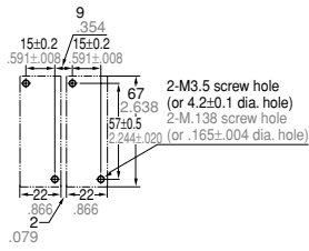
Mounting hole diagram HC2-Slim type
