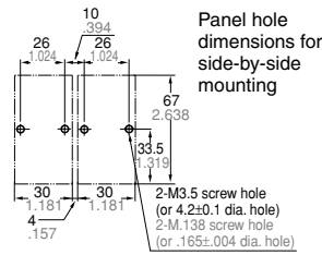
HC2, HC3 and HC4
