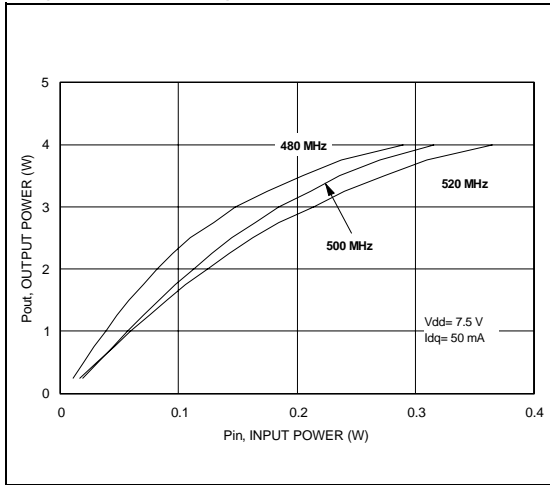
Output Power vs. Input Power PD54003
