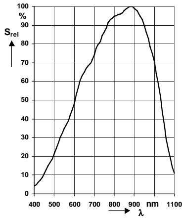
Photocurrent
