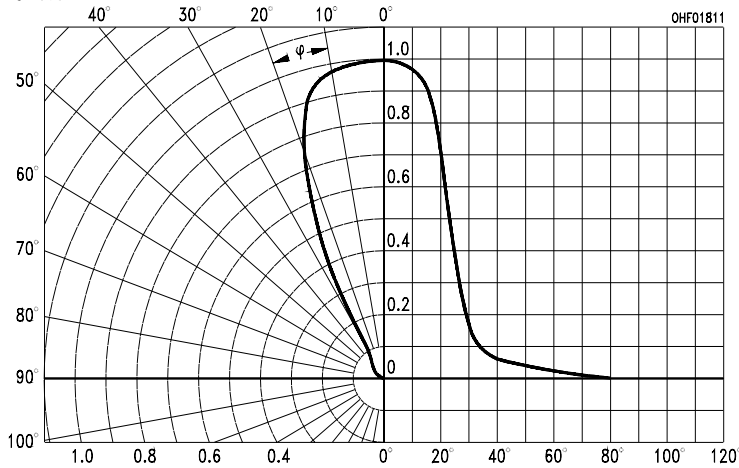
Directional Characteristics
