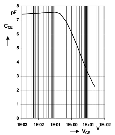
Collector-Emitter Capacitance
