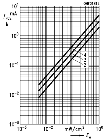
Photocurrent
