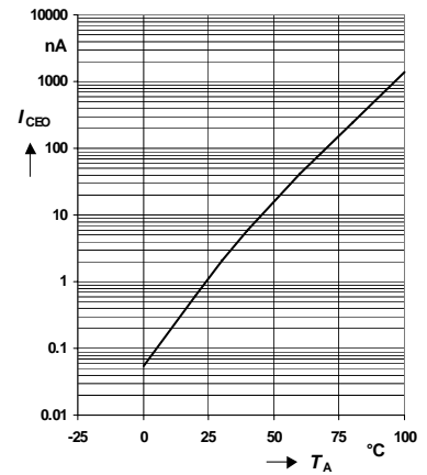
Dark Current
