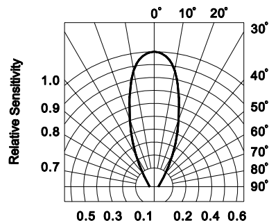
FIG.5 SENSITIVITY DIAGRAM
