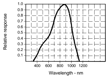
Fig. 4 Spectral Responsivity
