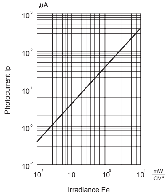
Figure 6. PHOTOCURRENT VS IRRADIANCE = 940 nm
