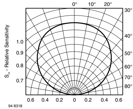
Figure 6. Relative Radiant Sensitivity vs. Angular Displacement
