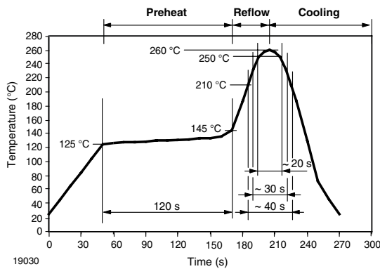
Figure 7. Tin (Sn) Reflow Solder Profile (Pb-free)
