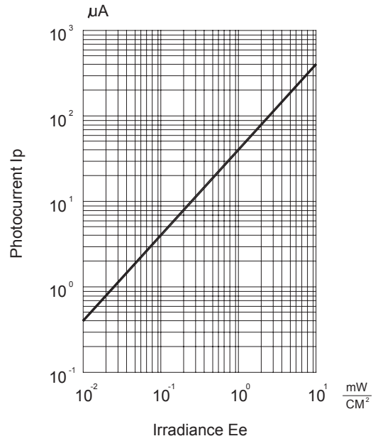
Figure 6. PHOTOCURRENT VS IRRADIANCE = 940 nm
