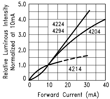
Fig.13 RELATIVE LUMINOUS INTENSITY VS. FORWARD CURRENT
