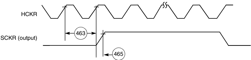
Figure 3-35 ESAL HCKR Timing
