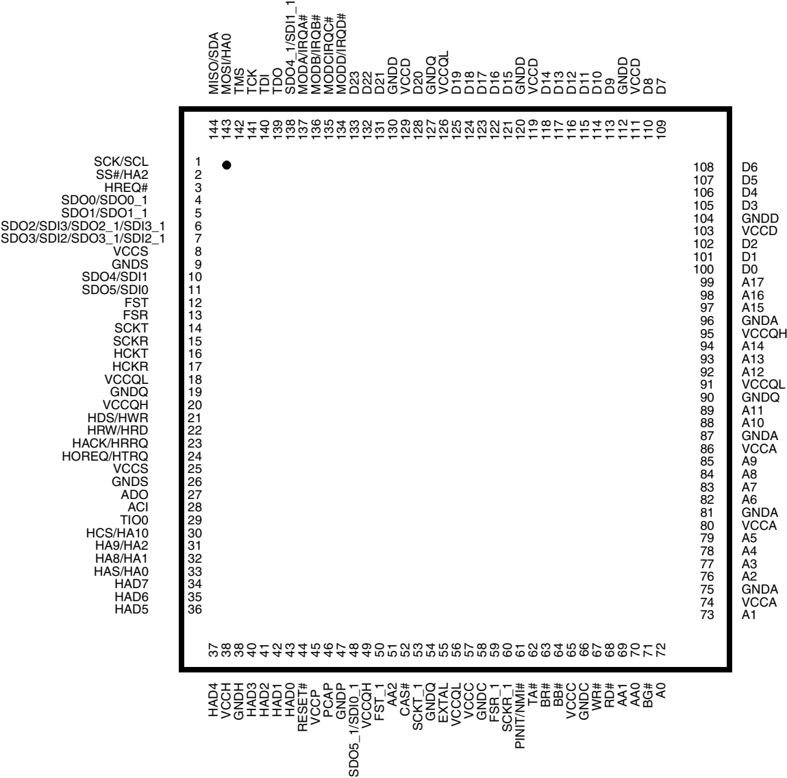
Figure 4-1 144-pin package
