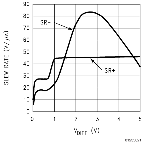
FIGURE 2. Slew Rate vs. V_{DIFF}
