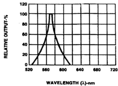
Fig.2 SPECTRAL RESPONSE
