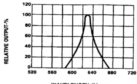
Fig.2 SPECTRAL RESPONSE
