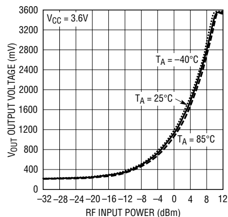
Typical Detector Characteristics, 3000MHz, Gain = 2, V_{OS} = 0\text{V}
