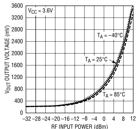
Typical Detector Characteristics, 6000MHz, Gain = 2, V_{OS} = 0\text{V}
