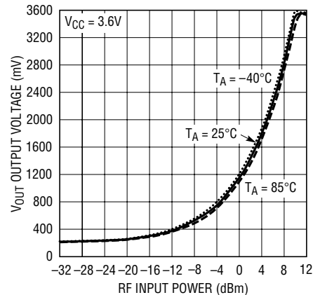
Typical Detector Characteristics, 600MHz, Gain = 2, V_{OS} = 0\text{V}
