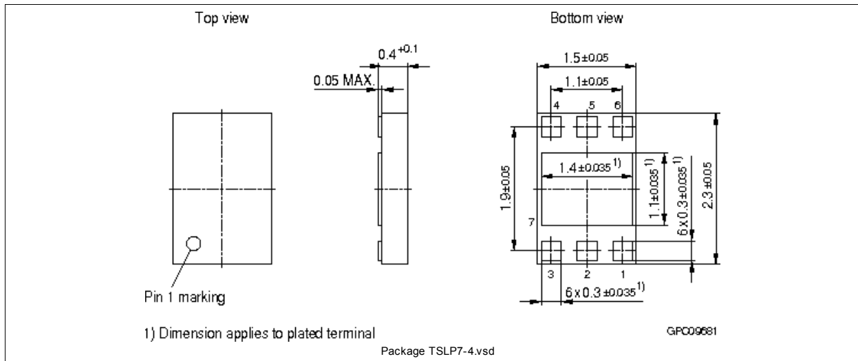
Figure 6 Package TSLP7-4
