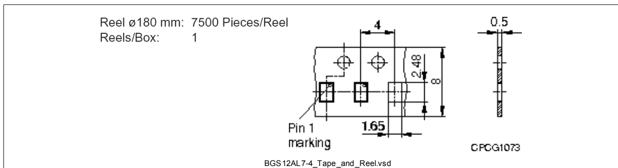
Figure 8 Tape and Reel
