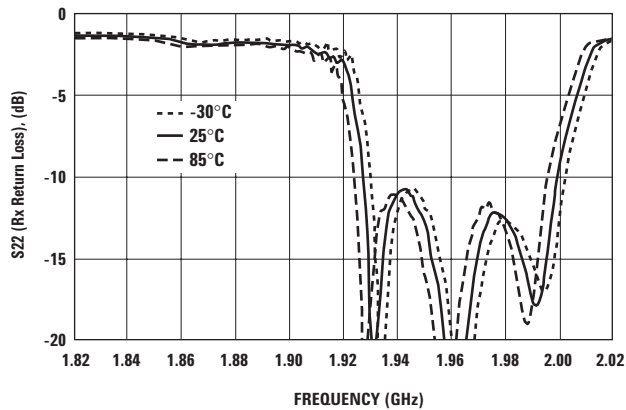
Figure 6. Return loss, Rx port.
