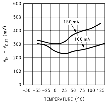
Minimum Input Voltage vs Temperature
